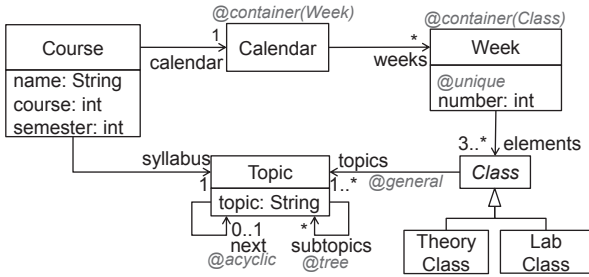
Fig. 17 Resulting meta-model.
